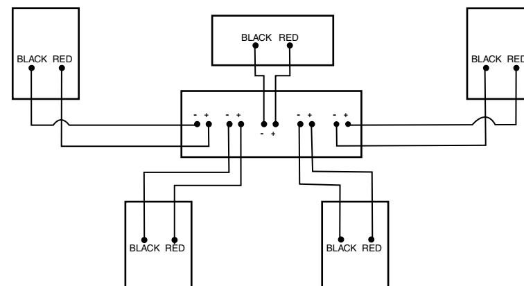
FIGURE 4 Connecting Speakers to Amplifier or Receiver
